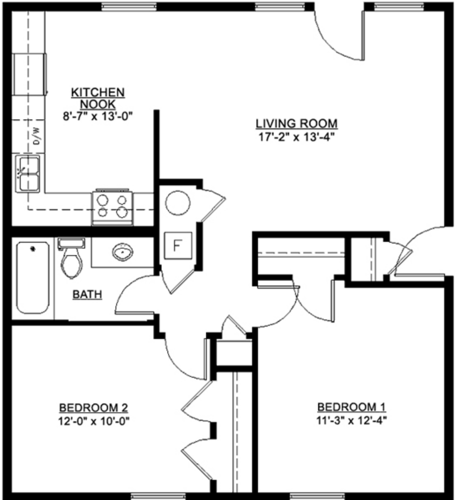
2 Bedroom Garden 757 Square Feet
